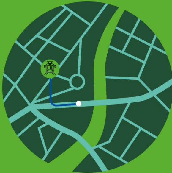
Single modal
